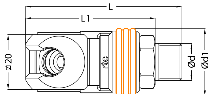
Socket / Kupplung
