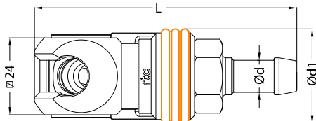
Socket / Kupplung
