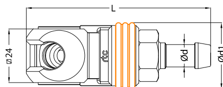
Socket / Kupplung
