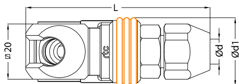
Socket / Kupplung
