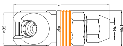
Socket / Kupplung
