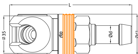
Socket / Kupplung
