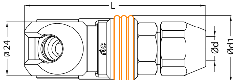
Socket / Kupplung
