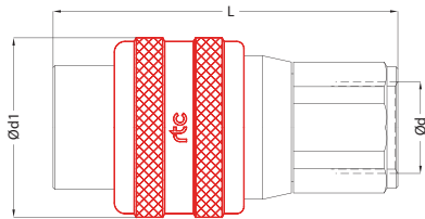
Socket / Kupplung
