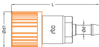
Socket / Kupplung
