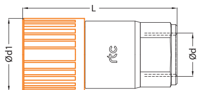
Socket / Kupplung
