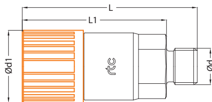
Socket / Kupplung
