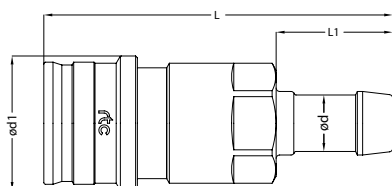
Socket / Kupplung
