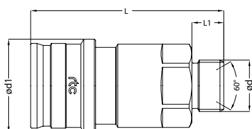
Socket / Kupplung
