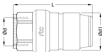
Plug Profile: 152.32 - 152.38 - 152.50
