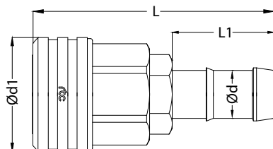
Socket / Kupplung
