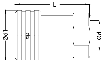
Double Shut-off
