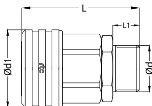
Socket / Kupplung
