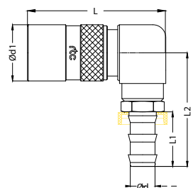
Socket / Kupplung
