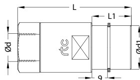
Socket / Kupplung
