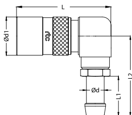
Socket / Kupplung
