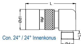
Socket / Kupplung
