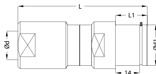
Socket / Kupplung
