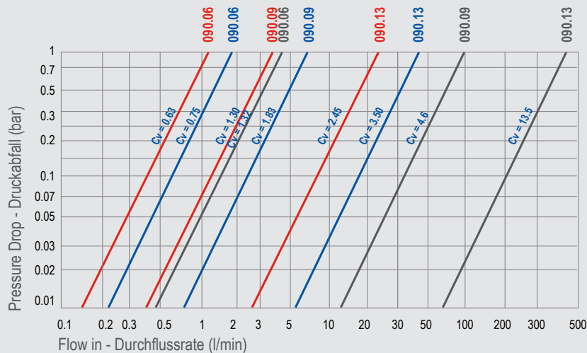
Flow Rate vs Pressure Drop Graph
