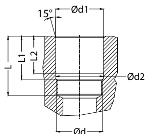
Socket / Kupplung
