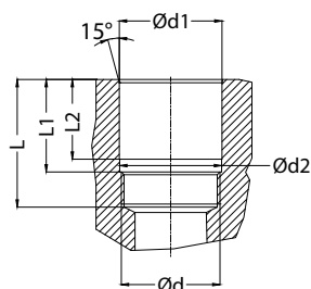
Socket / Kupplung
