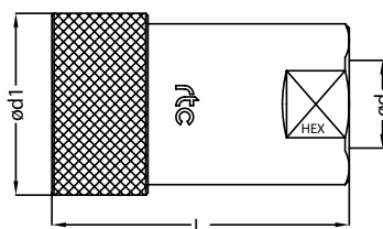
Socket / Kupplung
