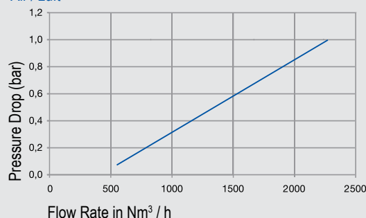
Flow Rate vs Pressure Drop Graph
