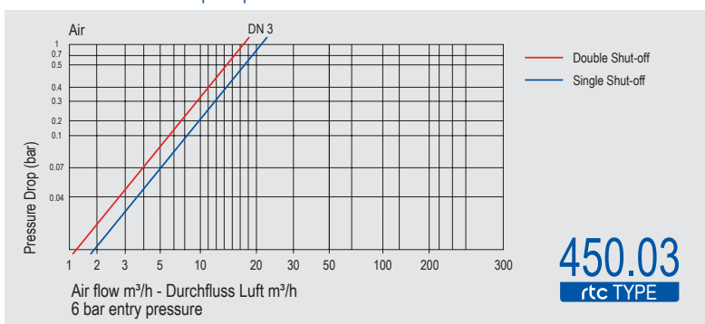
Flow Rate vs Pressure Drop Graph
